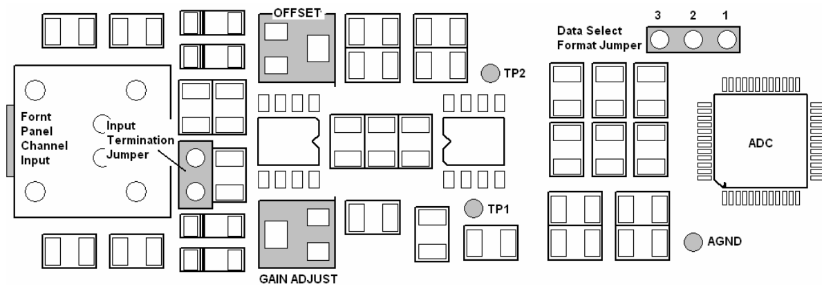
PCB Layout of a single channel
